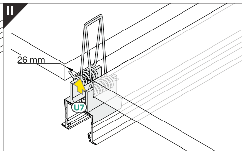
cone U7 mounting plate uchwyt U7 cone
